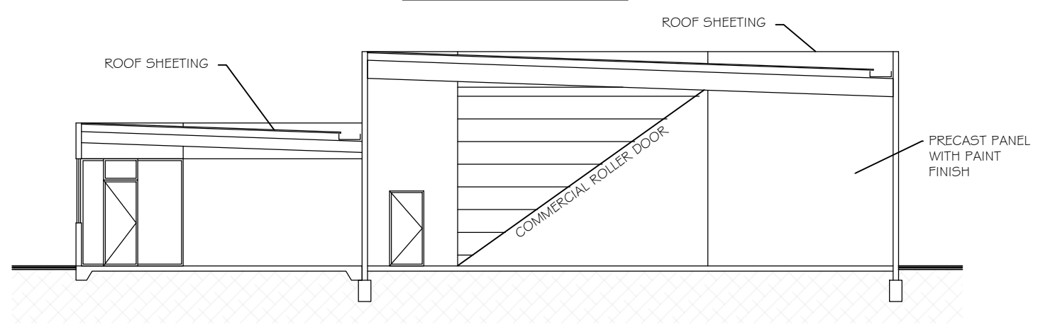
EAST ELEVATION
