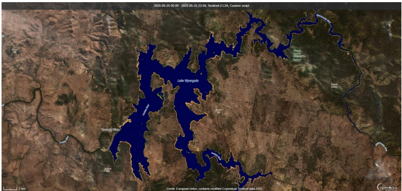
Figure 1. Wyangala Dam 25/5/2025 Sentinel Hub [CC BY-NC 4.0] NSW-Custom Algae Script - TF, WaterNSW
