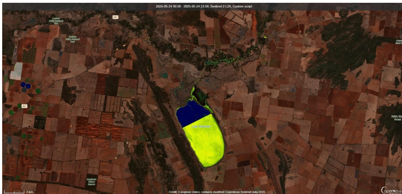
Figure 4. Lake Brewster 24/5/2025 Sentinel Hub [CC BY-NC 4.0] NSW-Custom Algae Script - TF, WaterNSW.
