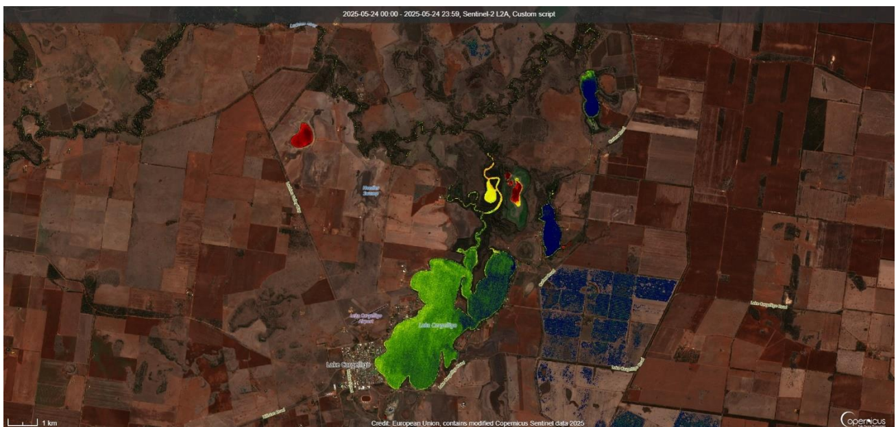
Figure 3. Lake Cargelligo 24/5/2025 Sentinel Hub [CC BY-NC 4.0] NSW-Custom Algae Script - TF, WaterNSW
