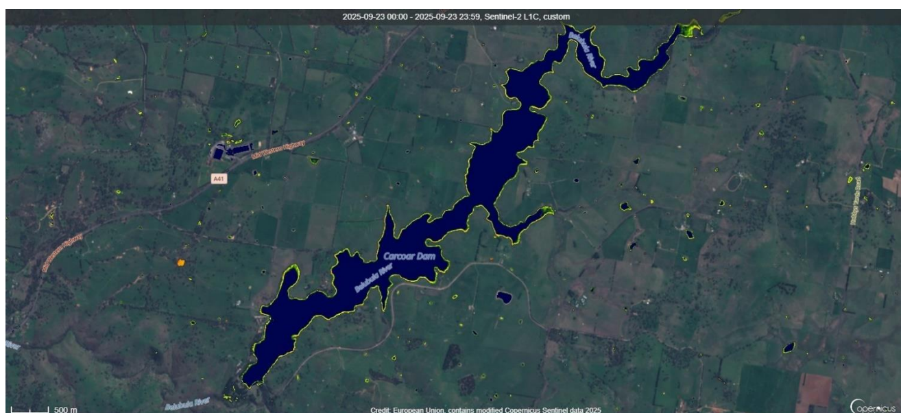
Figure 2. Carcoar Dam 23/9/2025 Sentinel Hub [CC BY-NC 4.0] NSW-Custom Algae Script - TF, WaterNSW
