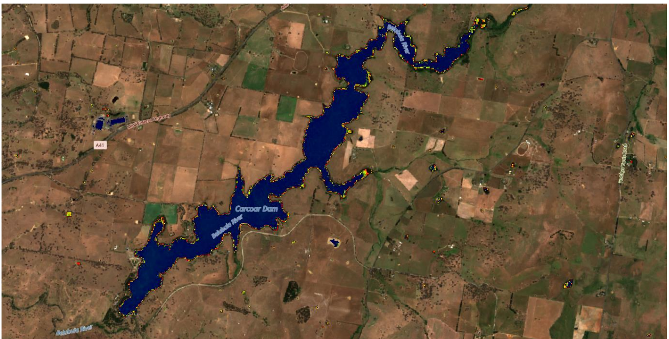
Figure 2. Carcoar Dam 08/01/2026 Sentinel Hub [CC BY-NC 4.0] NSW-Custom Algae Script - TF, WaterNSW
