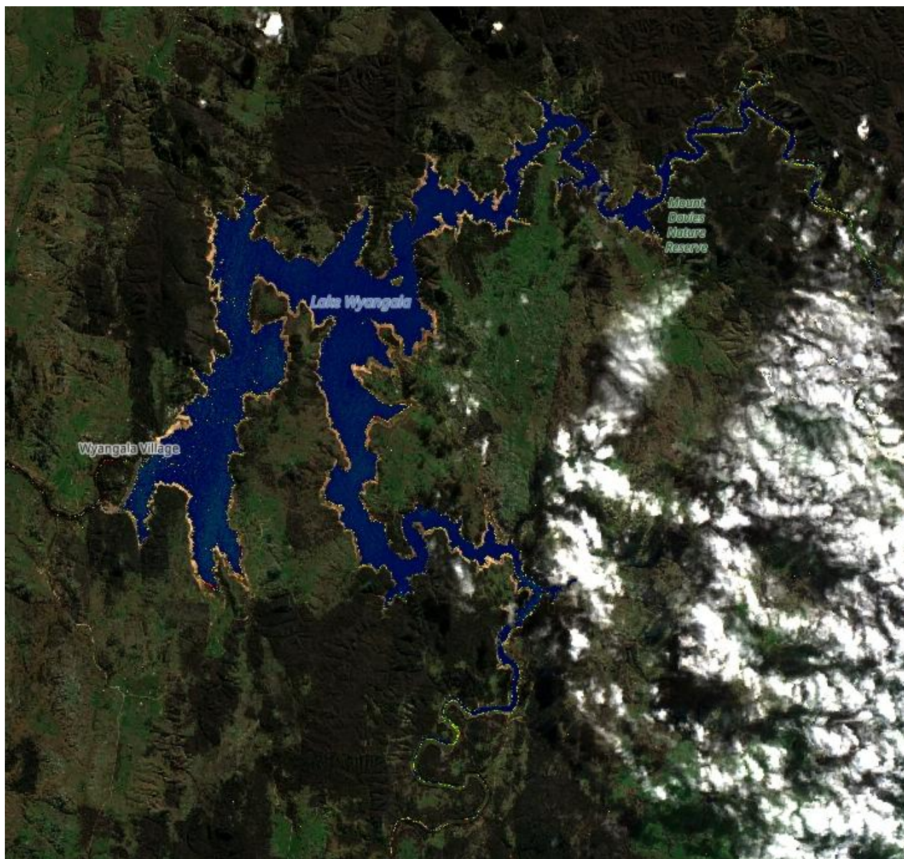
Figure 1. Wyangala Dam 25/06/2026 Sentinel Hub [CC BY-NC 4.0] NSW-Custom Algae Script - TF, WaterNSW
