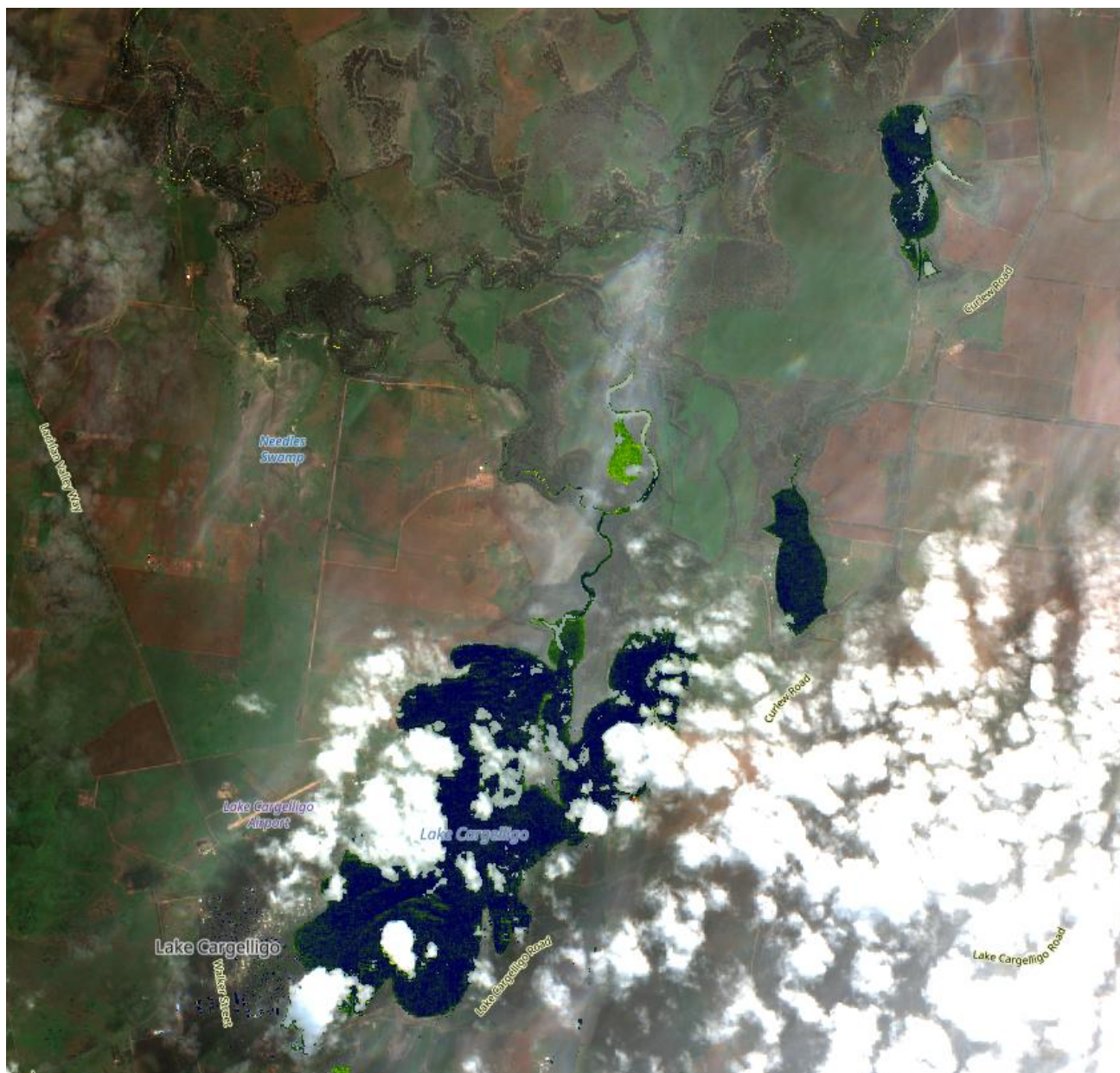
Figure 3. Lake Cargelligo 15/06/2026 Sentinel Hub [CC BY-NC 4.0] NSW-Custom Algae Script - TF, WaterNSW
