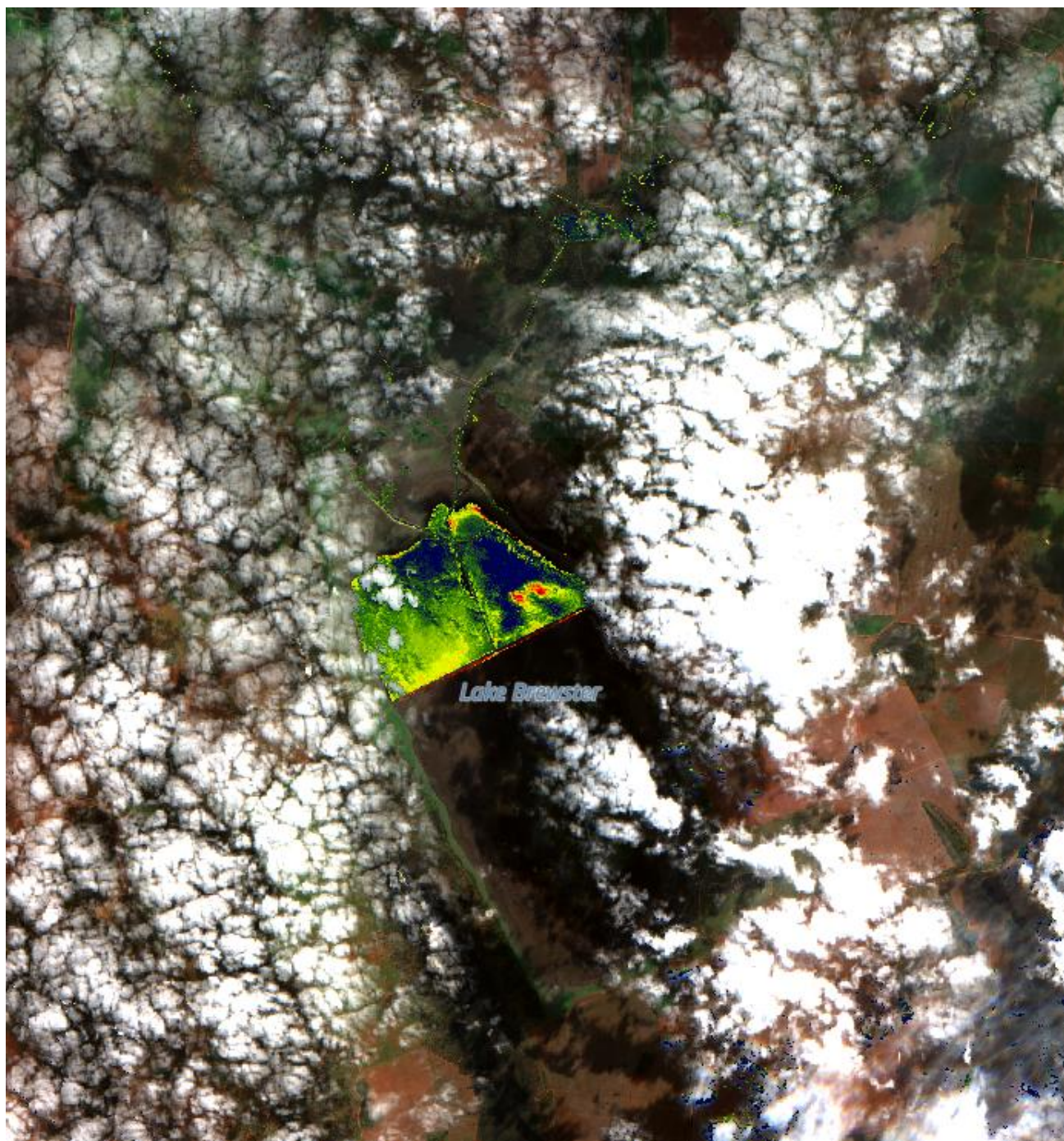
Figure 4. Lake Brewster 15/06/2026 Sentinel Hub [CC BY-NC 4.0] NSW-Custom Algae Script - TF, WaterNSW.
