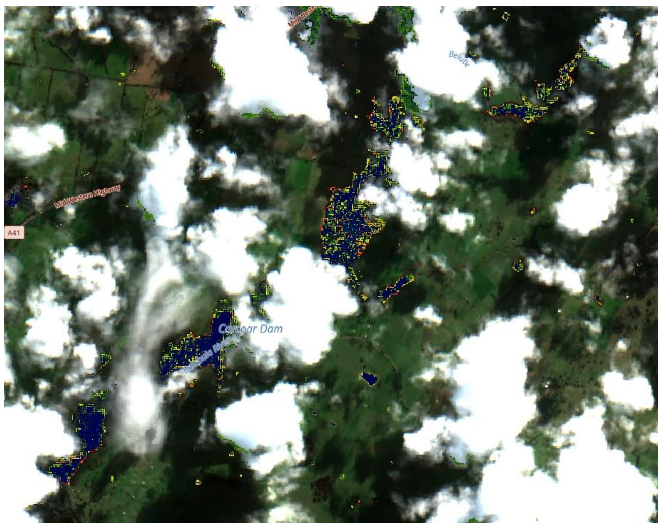
Figure 2. Carcoar Dam 22/06/2026 Sentinel Hub [CC BY-NC 4.0] NSW-Custom Algae Script - TF, WaterNSW
