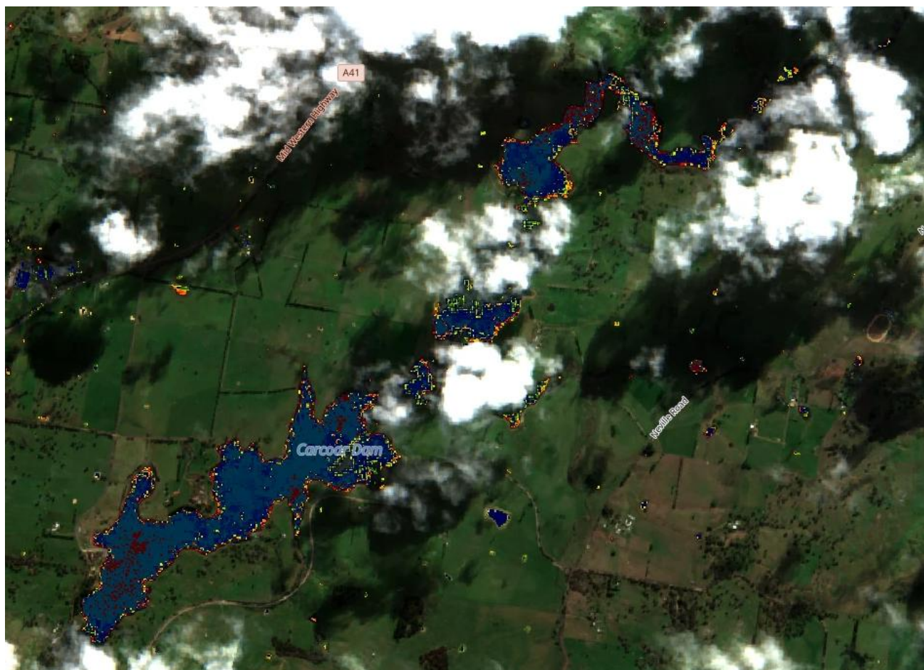
Figure 2. Carcoar Dam 17/07/2026 Sentinel Hub [CC BY-NC 4.0] NSW-Custom Algae Script - TF, WaterNSW
