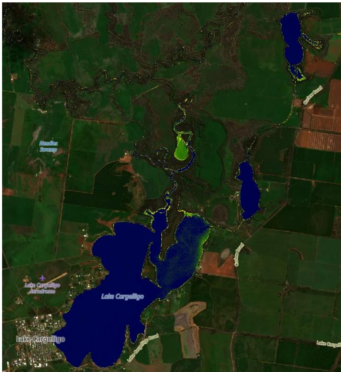
Figure 3. Lake Cargelligo 12/08/2026 Sentinel Hub [CC BY-NC 4.0] NSW-Custom Algae Script - TF, WaterNSW
